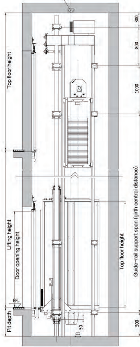
Vertical view of well side
