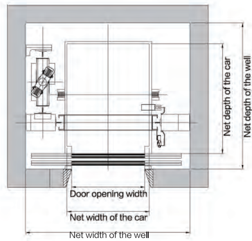
Well layout chart
