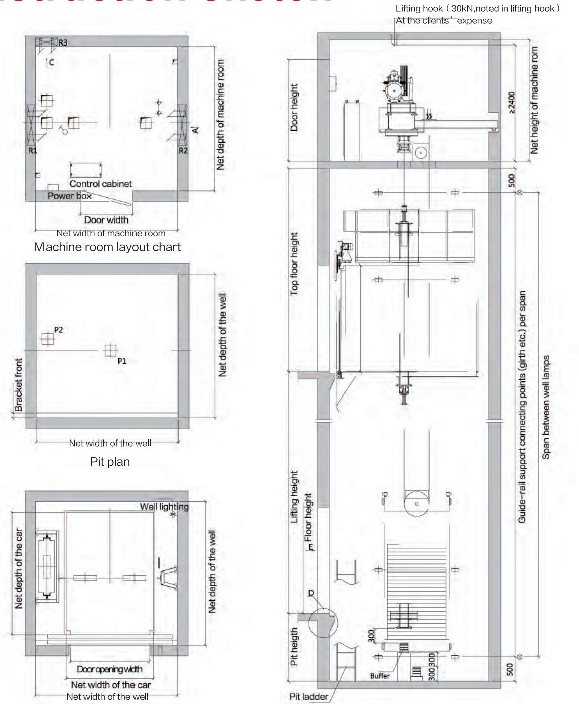
Well layout chart
