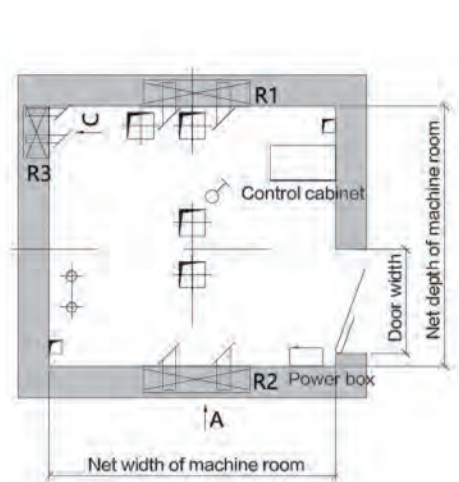
Machine room layout chart
